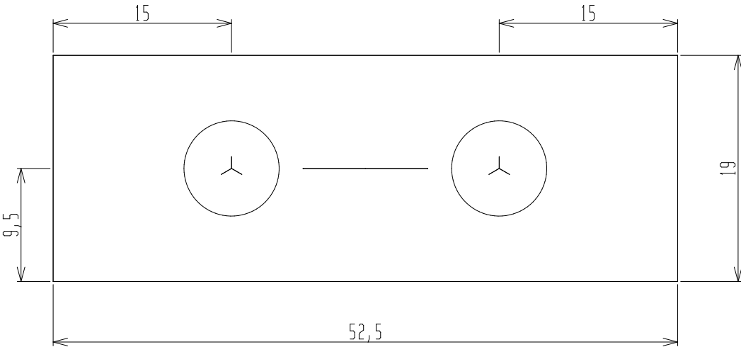
Steuntraver_02->ISO
